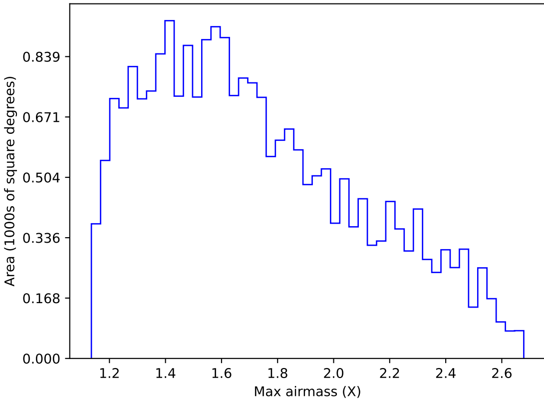
weather_cloudso18v3.4_10yrs Yr 1 y band: Max airmass
