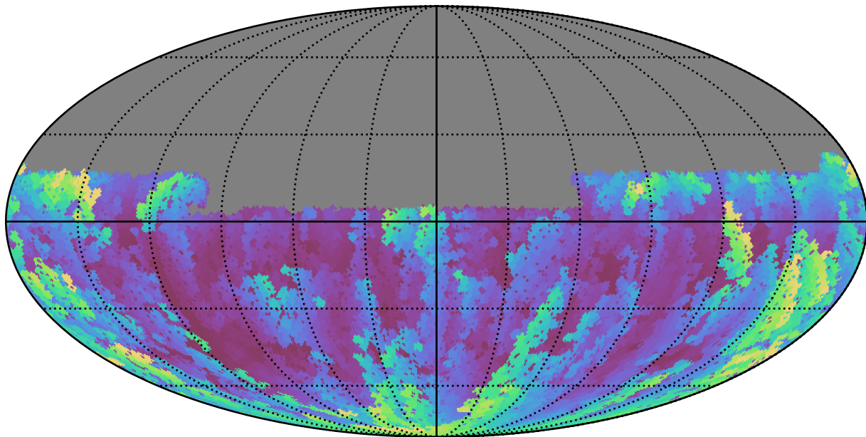
weather_cloudso18v3.4_10yrs Yr 1 u band: Max airmass
