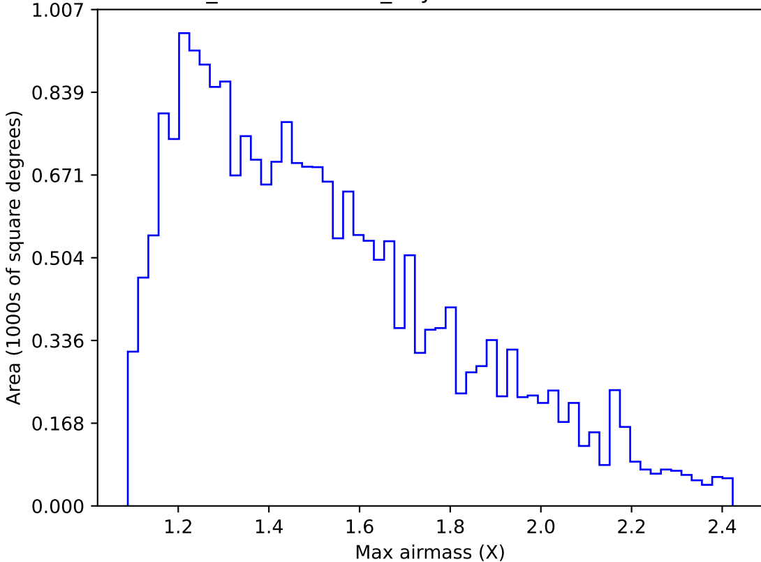
weather_cloudso18v3.4_10yrs Yr 1 u band: Max airmass
