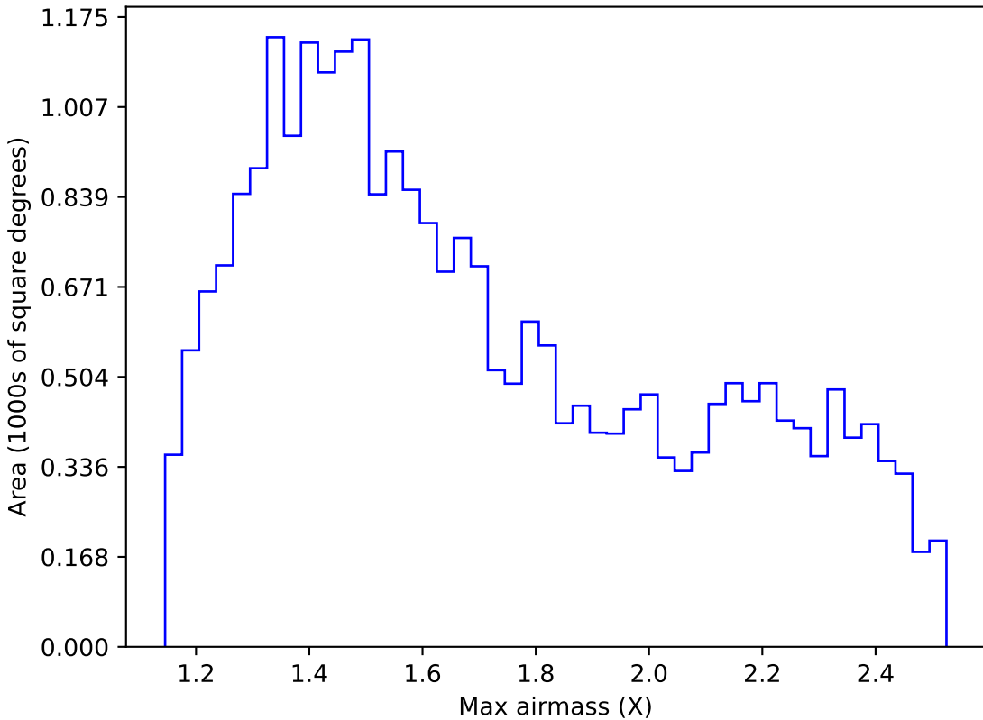
weather_cloudso18v3.4_10yrs Yr 1 r band: Max airmass
