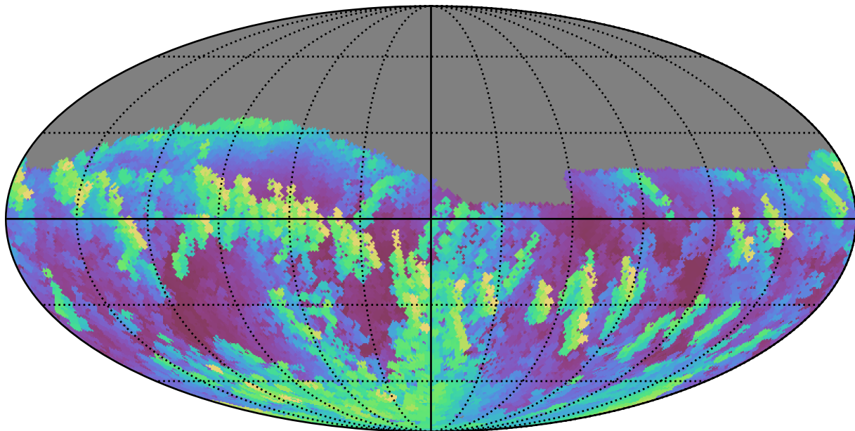
weather_cloudso18v3.4_10yrs Yr 1 i band: Max airmass
