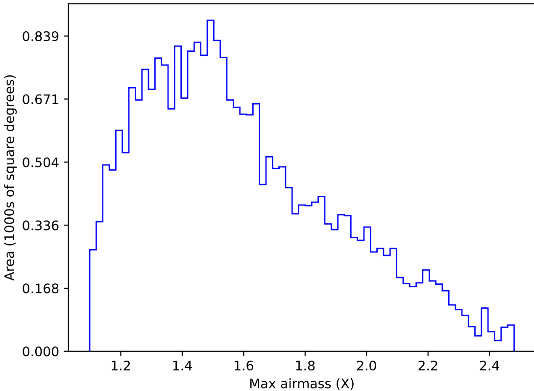
weather_cloudso18v3.4_10yrs Yr 1 g band: Max airmass
