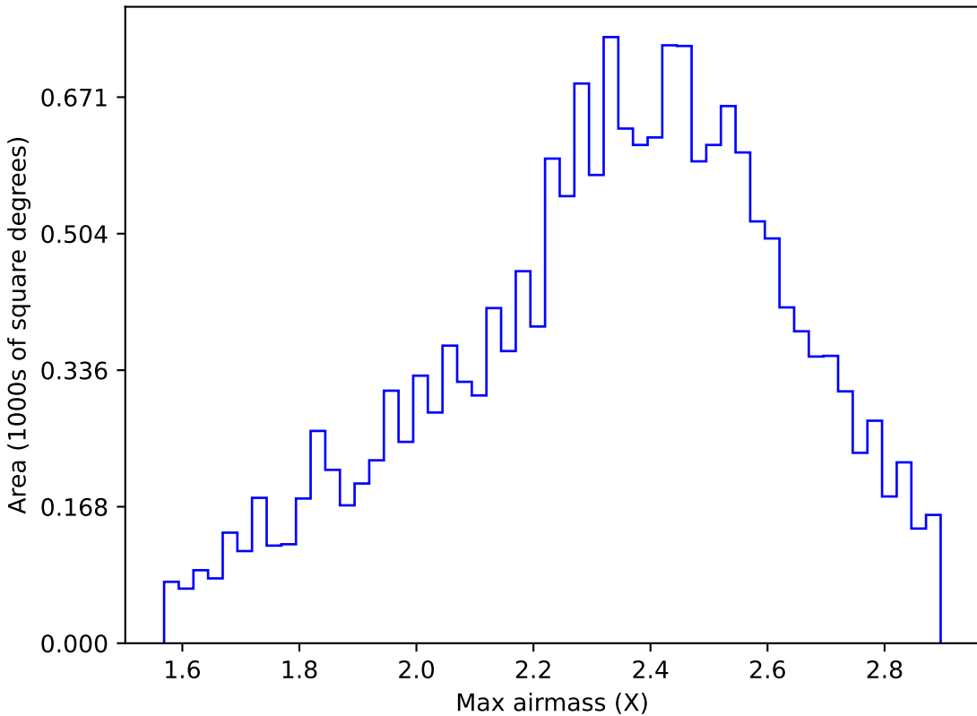
weather_cloudso18v3.4_10yrs WFD y band: Max airmass
