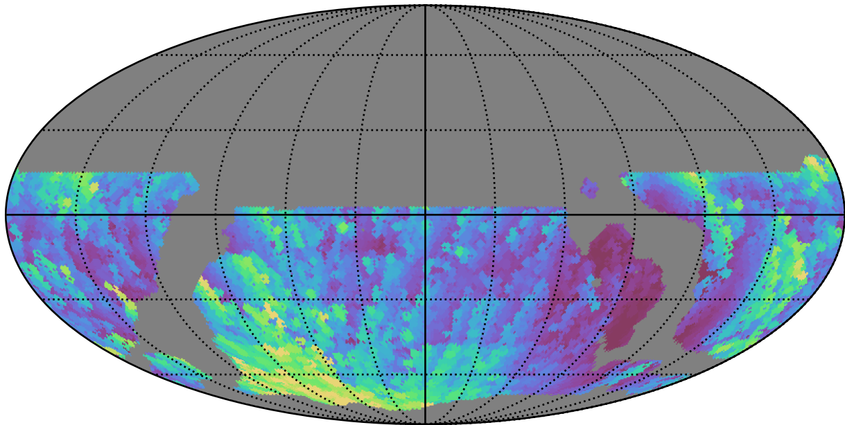
weather_cloudso18v3.4_10yrs WFD u band: Max airmass
