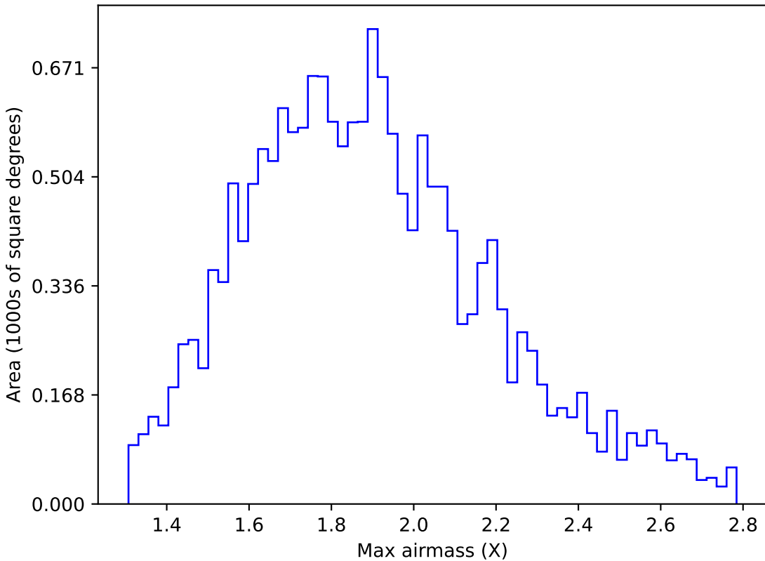
weather_cloudso18v3.4_10yrs WFD u band: Max airmass
