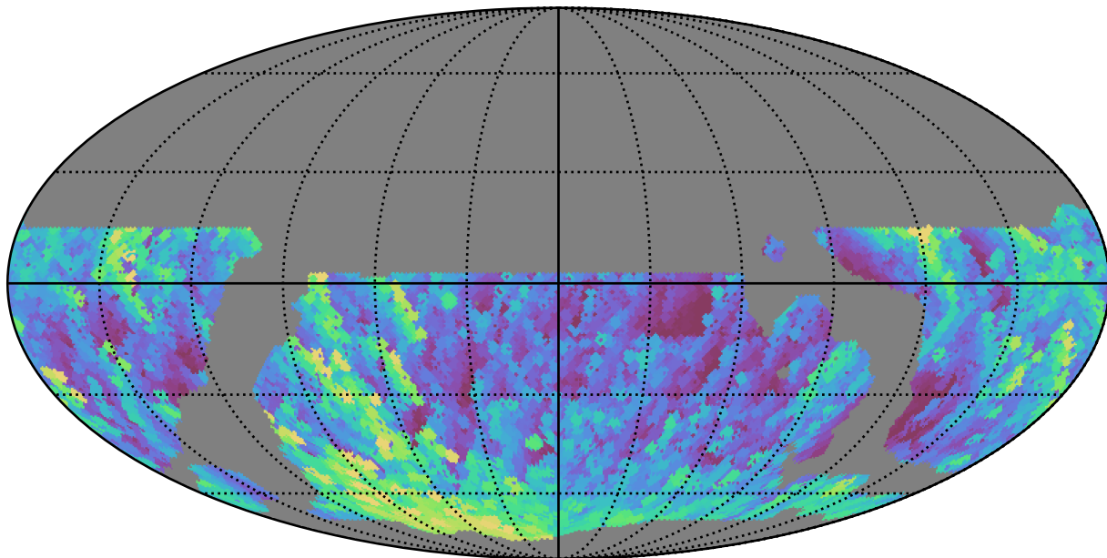
weather_cloudso18v3.4_10yrs WFD g band: Max airmass
