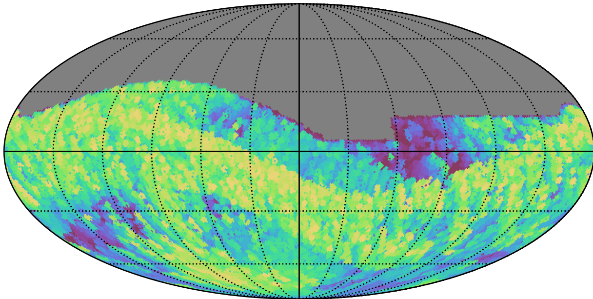
weather_cloudso18v3.4_10yrs All sky z band: Max airmass
