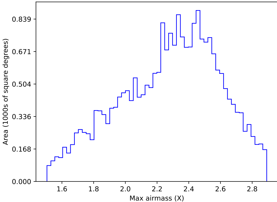
weather_cloudso18v3.4_10yrs All sky y band: Max airmass
