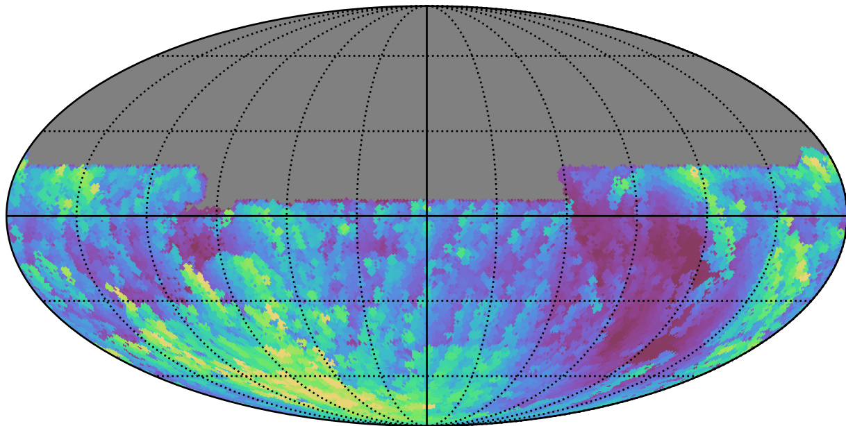
weather_cloudso18v3.4_10yrs All sky u band: Max airmass
