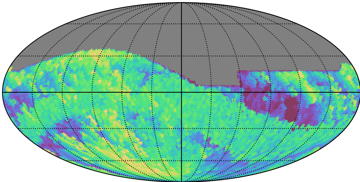
weather_cloudso18v3.4_10yrs All sky r band: Max airmass
