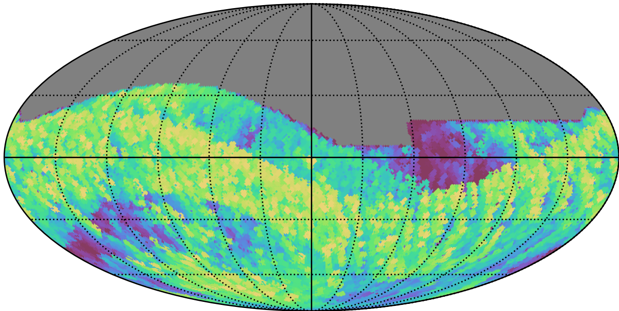
weather_cloudso18v3.4_10yrs All sky i band: Max airmass
