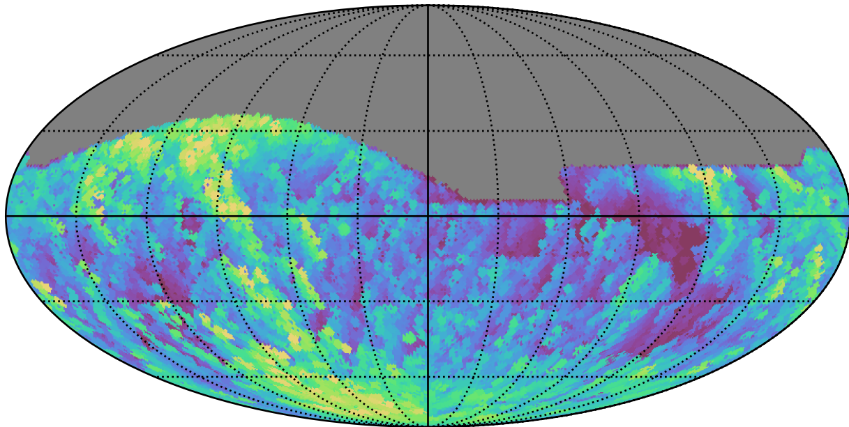
weather_cloudso18v3.4_10yrs All sky g band: Max airmass
