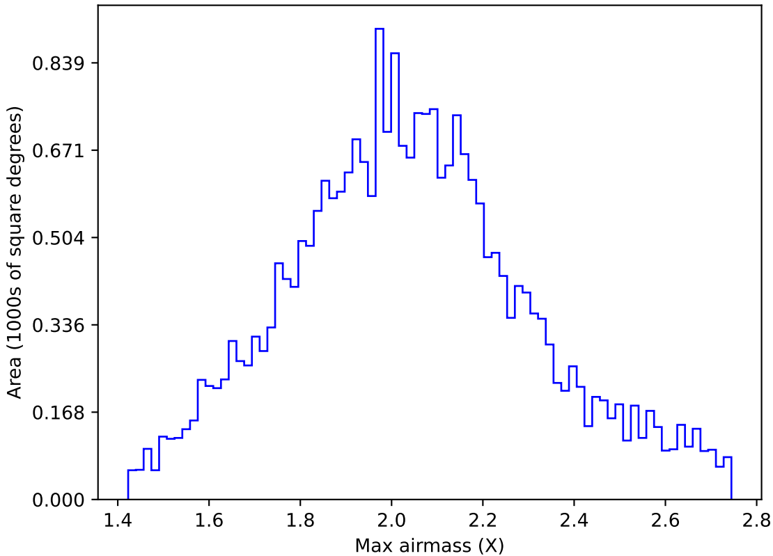
weather_cloudso18v3.4_10yrs All sky g band: Max airmass
