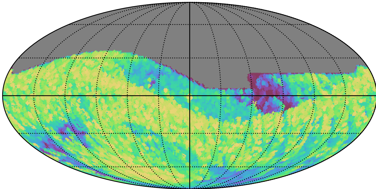
weather_cloudso18v3.4_10yrs All sky all bands: Max airmass
