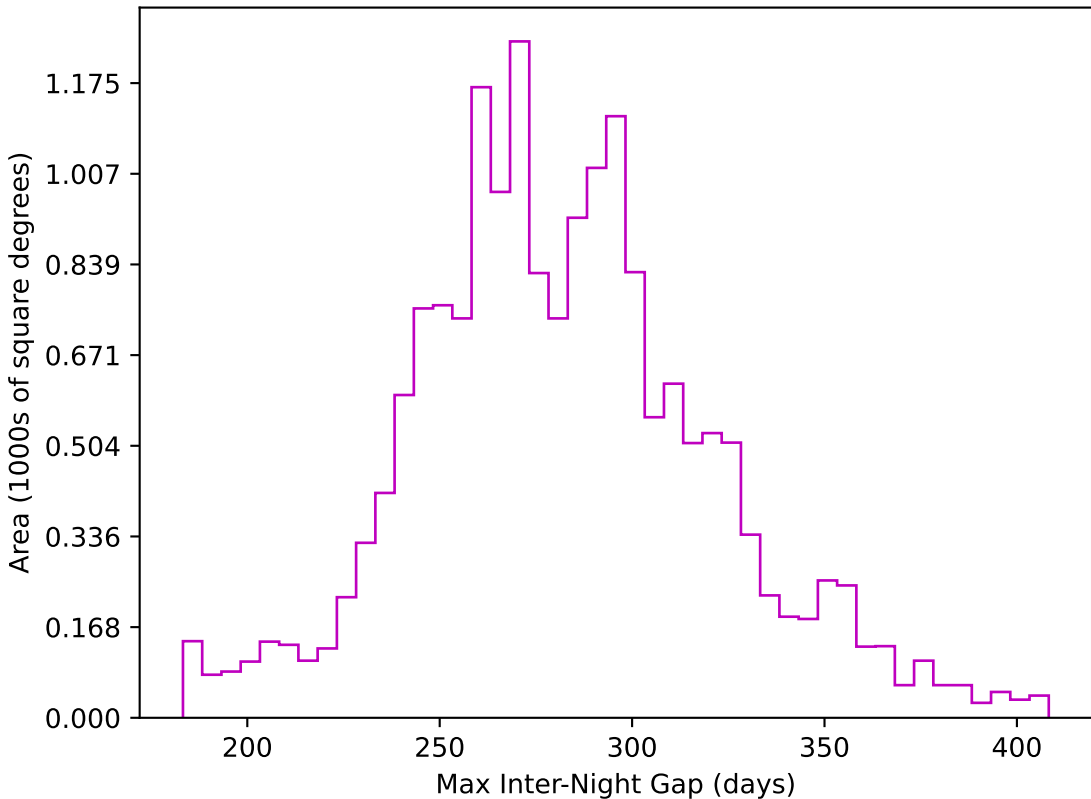
weather_cloudso18v3.4_10yrs WFD z band: Max Inter-Night Gap
