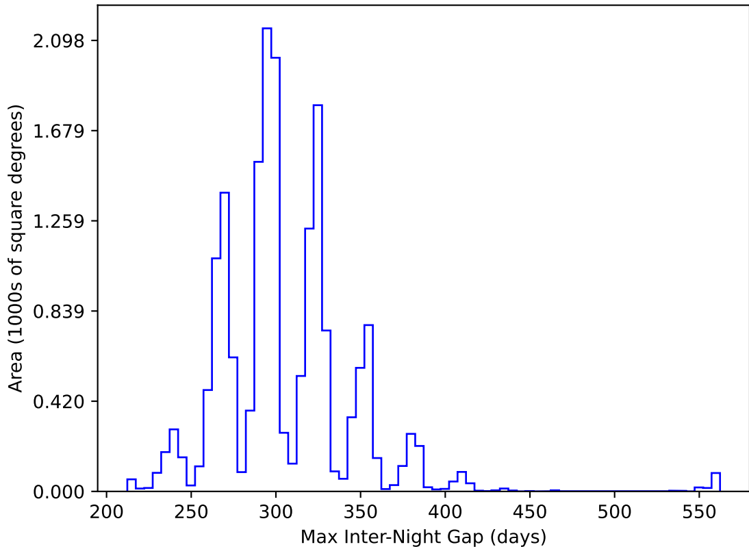
weather_cloudso18v3.4_10yrs WFD y band: Max Inter-Night Gap
