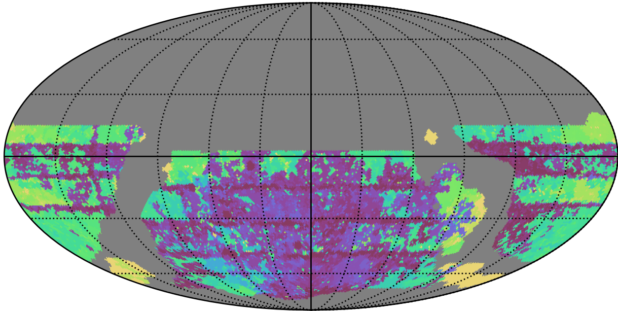
weather_cloudso18v3.4_10yrs WFD u band: Max Inter-Night Gap
