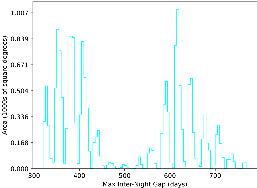
weather_cloudso18v3.4_10yrs WFD u band: Max Inter-Night Gap
