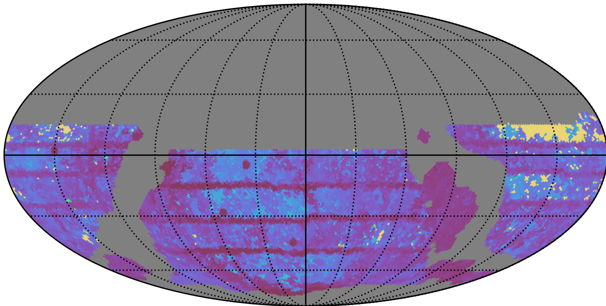
weather_cloudso18v3.4_10yrs WFD r band: Max Inter-Night Gap
