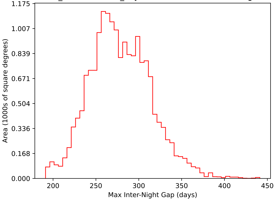
weather_cloudso18v3.4_10yrs WFD i band: Max Inter-Night Gap
