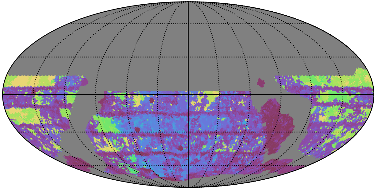
weather_cloudso18v3.4_10yrs WFD g band: Max Inter-Night Gap
