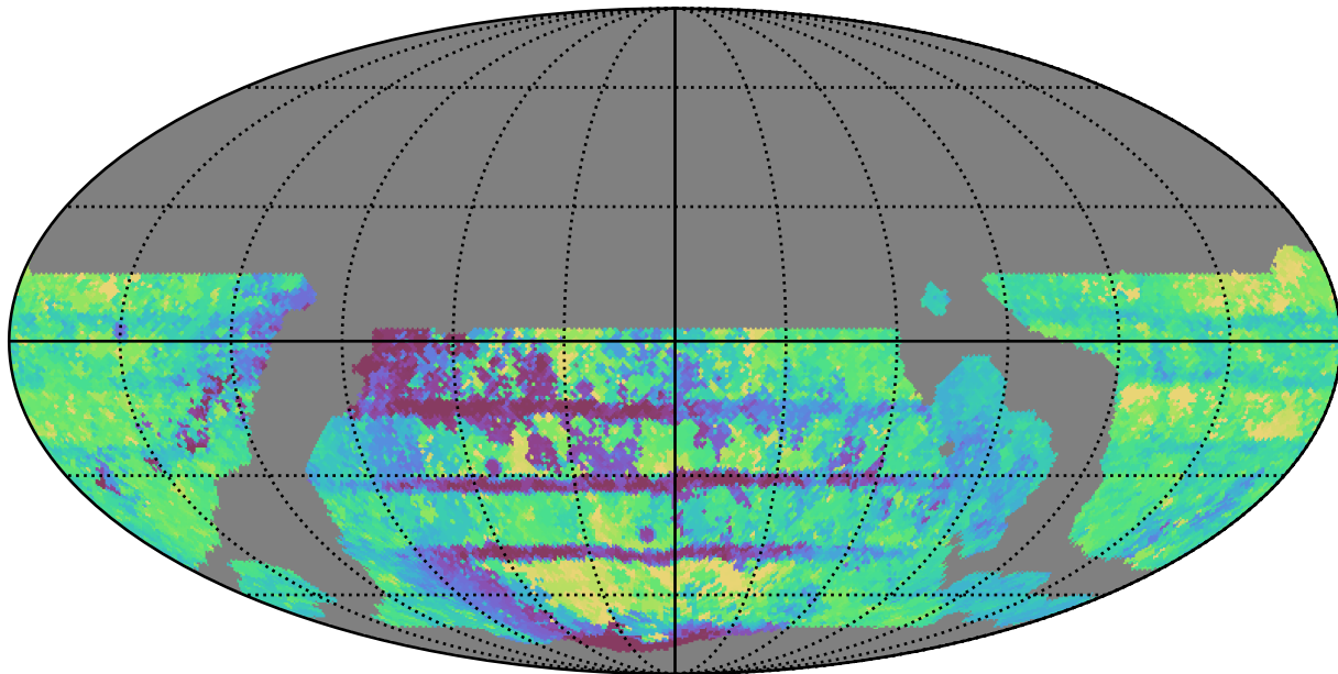
weather_cloudso18v3.4_10yrs WFD all bands: Max Inter-Night Gap
