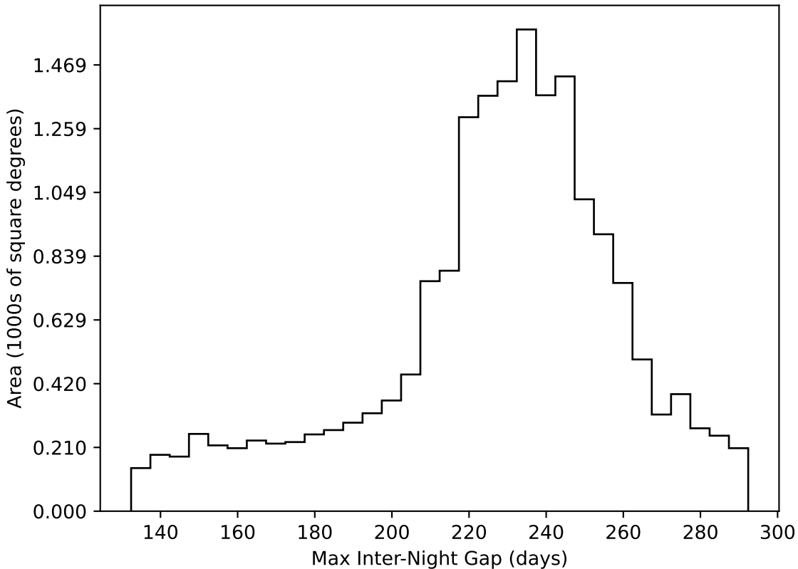
weather_cloudso18v3.4_10yrs WFD all bands: Max Inter-Night Gap
