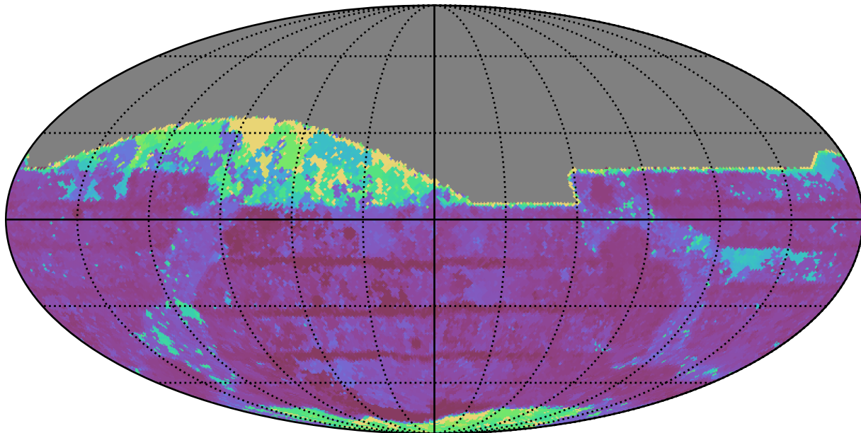
weather_cloudso18v3.4_10yrs All sky z band: Max Inter-Night Gap
