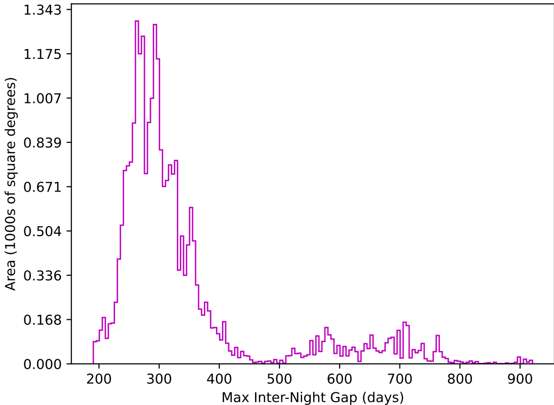
weather_cloudso18v3.4_10yrs All sky z band: Max Inter-Night Gap
