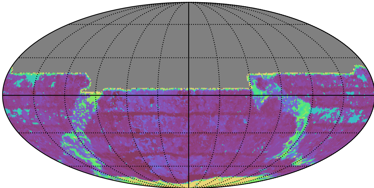
weather_cloudso18v3.4_10yrs All sky y band: Max Inter-Night Gap
