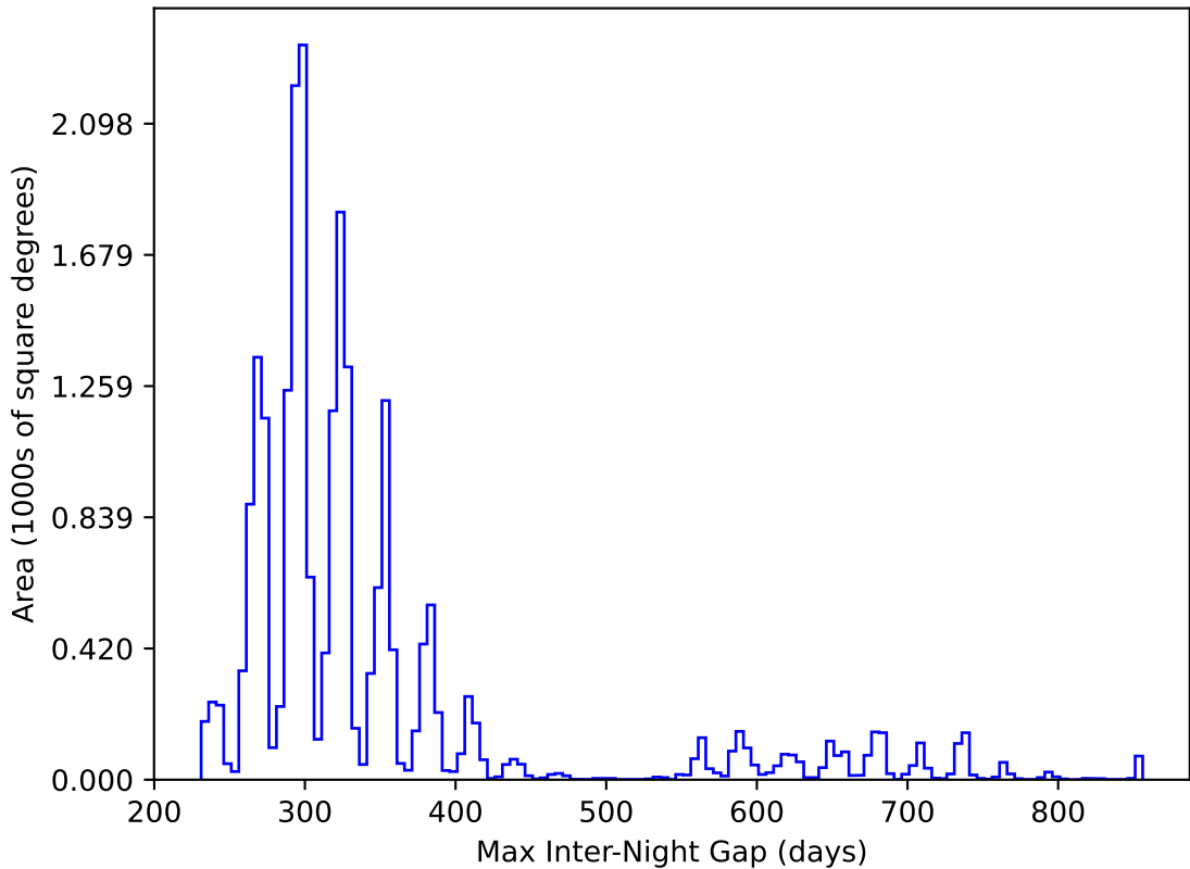
weather_cloudso18v3.4_10yrs All sky y band: Max Inter-Night Gap
