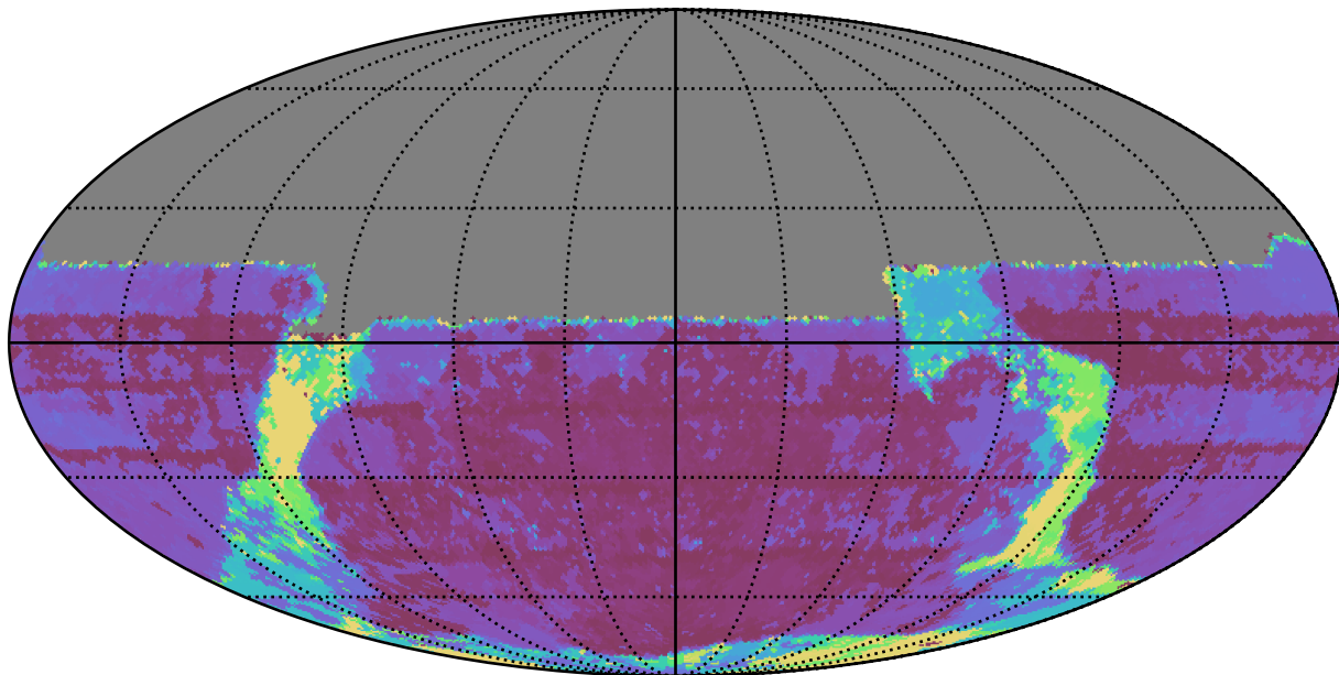
weather_cloudso18v3.4_10yrs All sky u band: Max Inter-Night Gap
