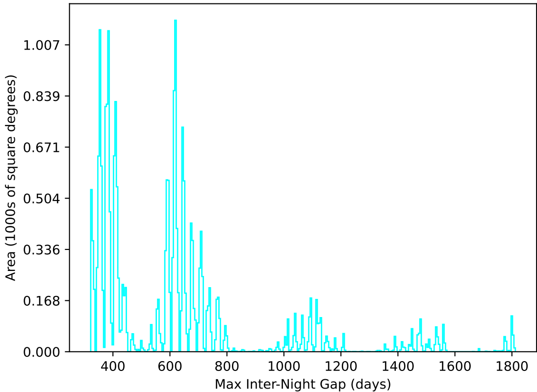
weather_cloudso18v3.4_10yrs All sky u band: Max Inter-Night Gap
