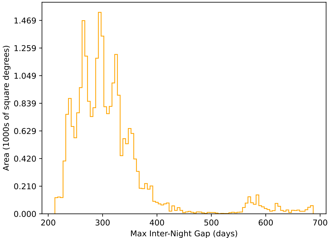
weather_cloudso18v3.4_10yrs All sky r band: Max Inter-Night Gap
