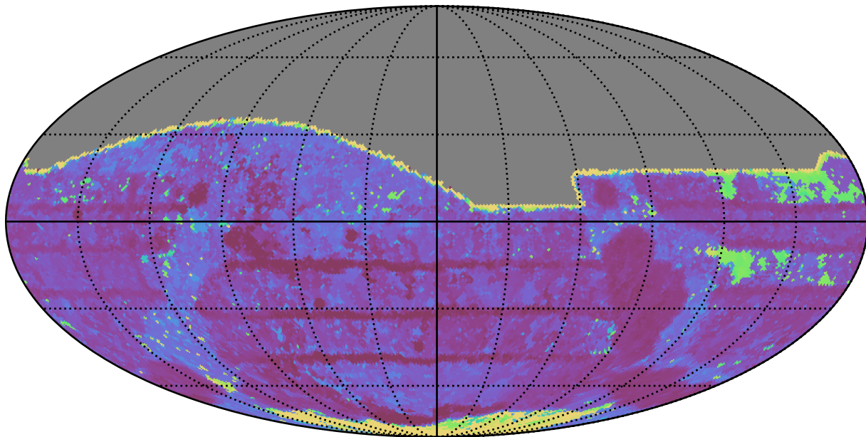
weather_cloudso18v3.4_10yrs All sky i band: Max Inter-Night Gap
