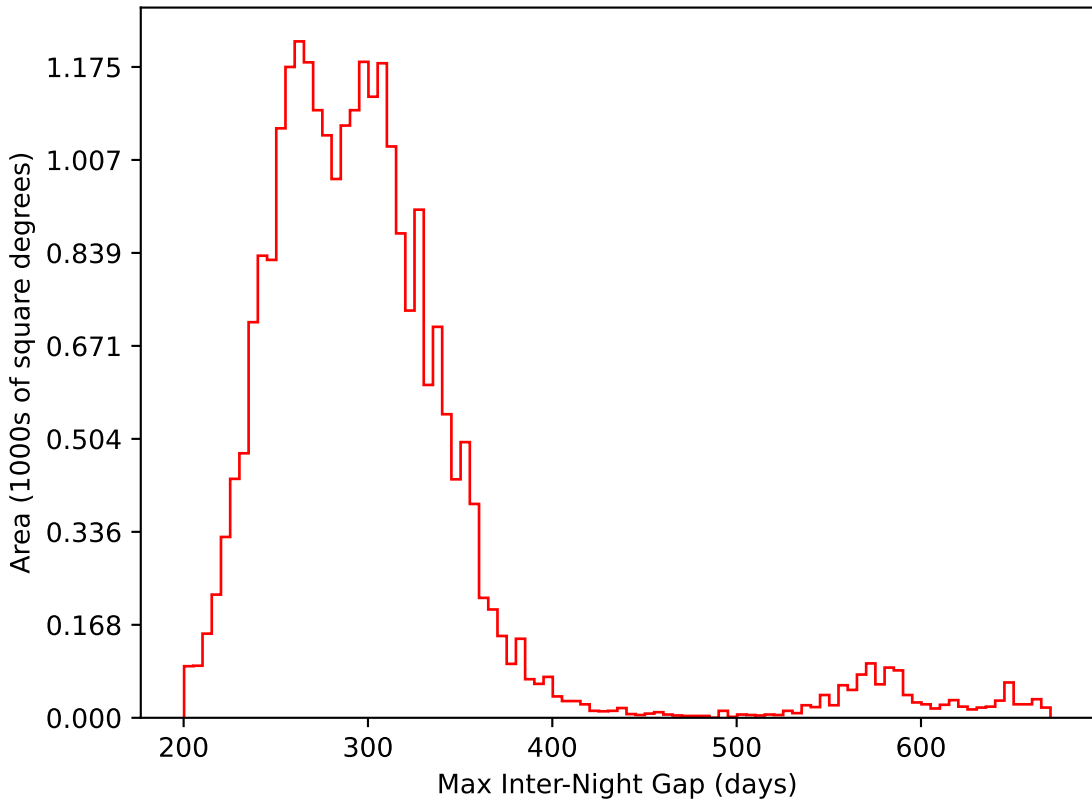
weather_cloudso18v3.4_10yrs All sky i band: Max Inter-Night Gap
