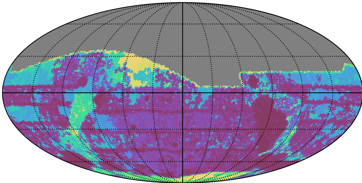
weather_cloudso18v3.4_10yrs All sky g band: Max Inter-Night Gap
