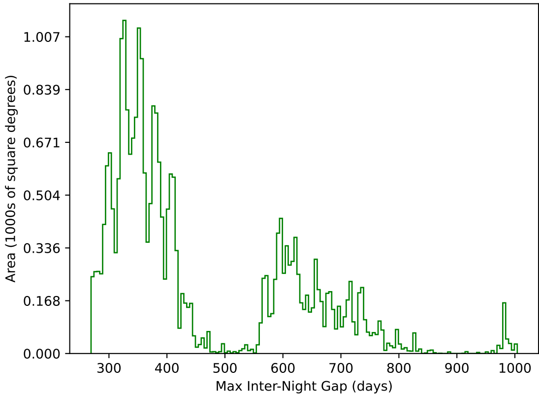
weather_cloudso18v3.4_10yrs All sky g band: Max Inter-Night Gap
