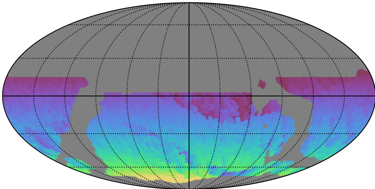
weather_cloudso18v3.4_10yrs WFD all bands: Max HA
