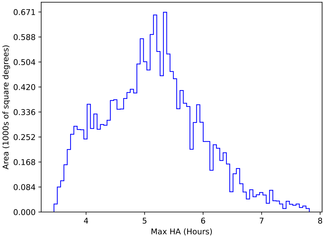
weather_cloudso18v3.4_10yrs WFD all bands: Max HA
