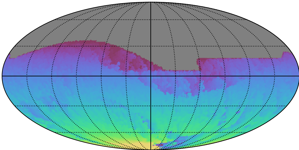
weather_cloudso18v3.4_10yrs All sky all bands: Max HA
