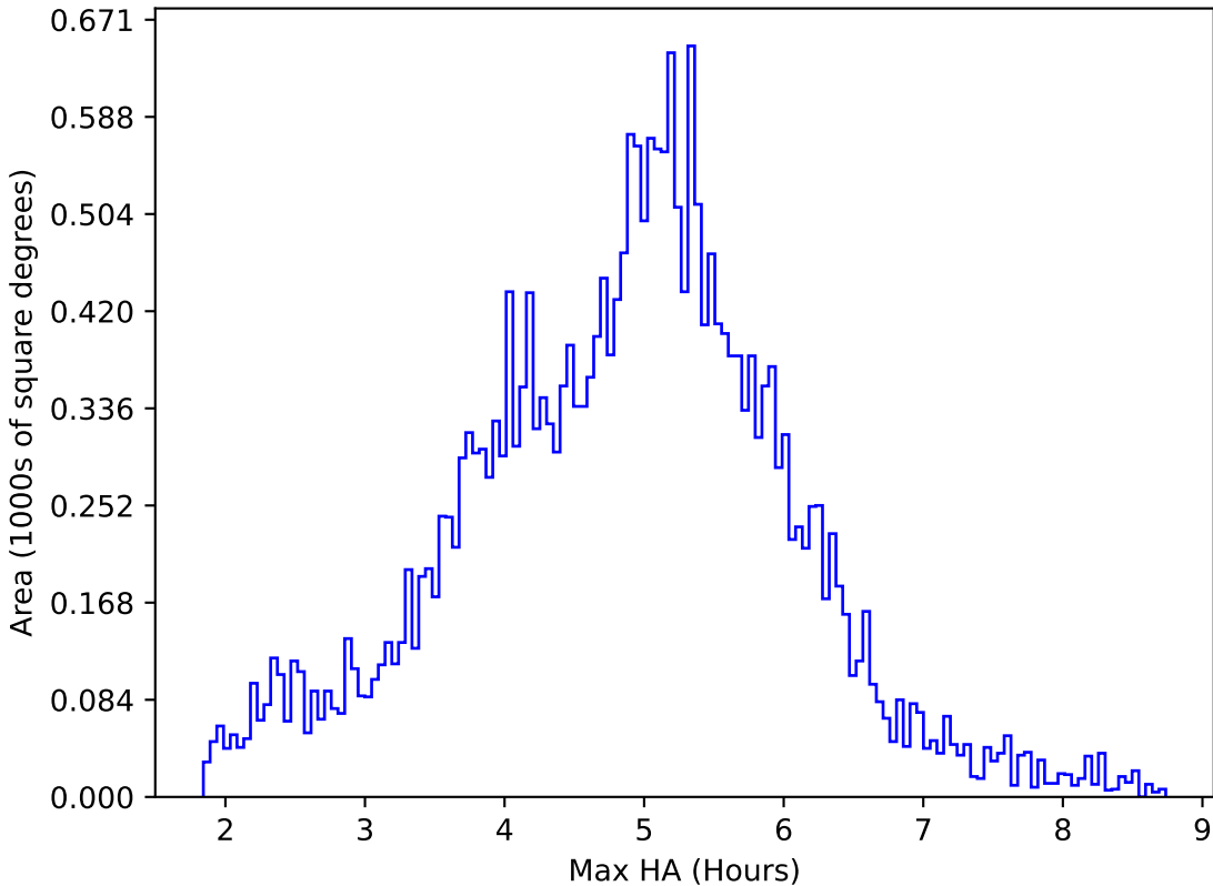
weather_cloudso18v3.4_10yrs All sky all bands: Max HA
