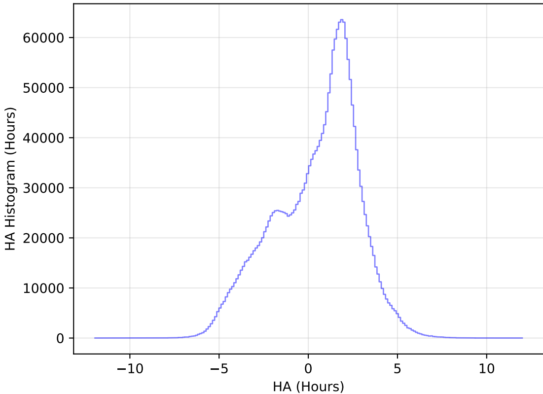
weather_cloudso18v3.4_10yrs WFD all bands: HA Histogram
