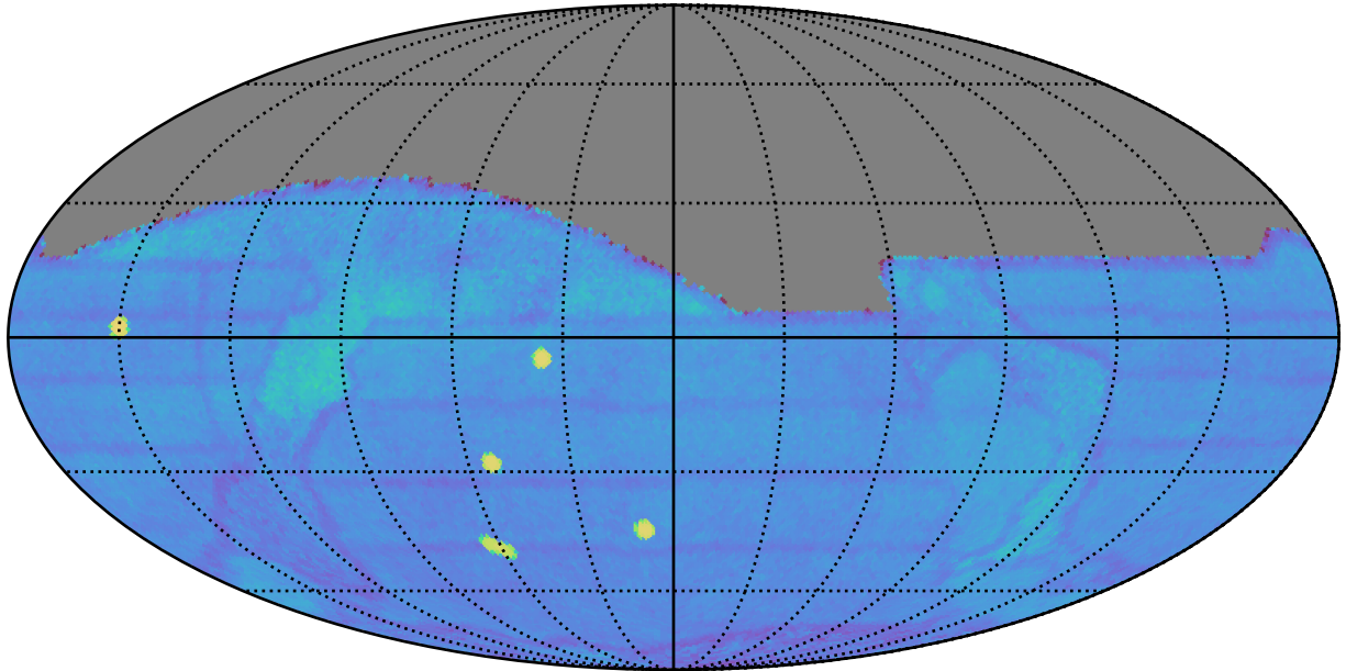
weather_cloudso18v3.4_10yrs gri All sky: Fraction of visits with a revisit < 60 min
