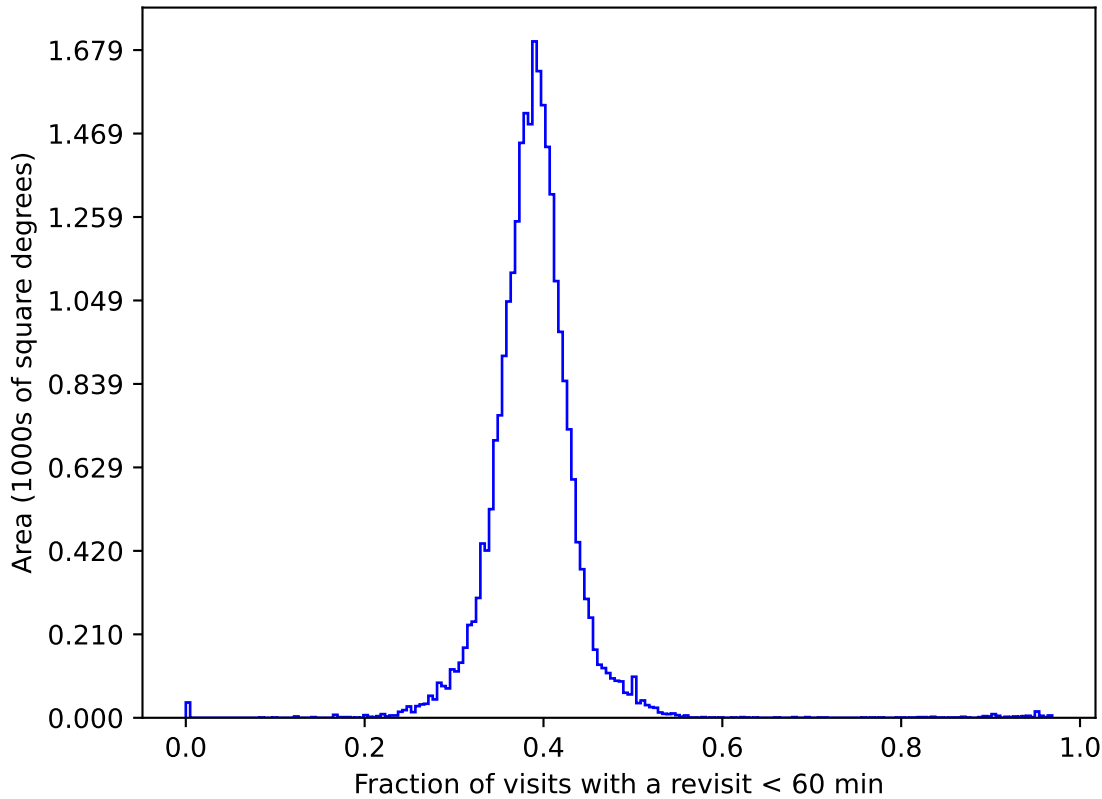
weather_cloudso18v3.4_10yrs gri All sky: Fraction of visits with a revisit < 60 min
