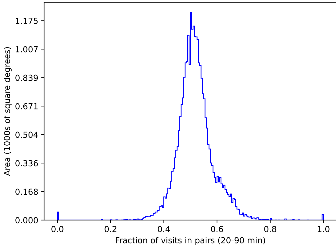
weather_cloudso18v3.4_10yrs gri All sky: Fraction of visits in pairs (20-90 min)
