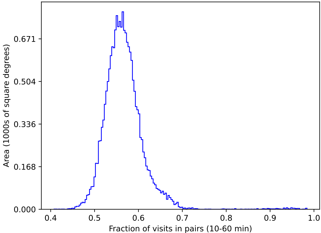
weather_cloudso18v3.4_10yrs gri WFD: Fraction of visits in pairs (10-60 min)
