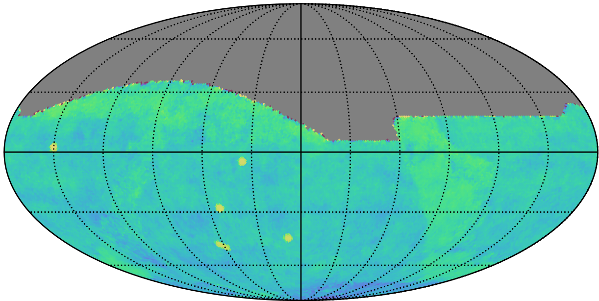
weather_cloudso18v3.4_10yrs gri All sky: Fraction of visits in pairs (10-60 min)
