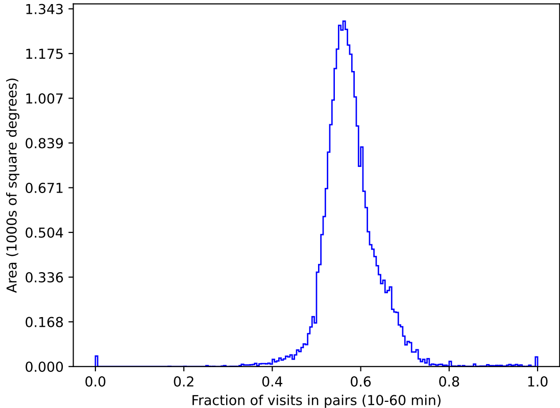
weather_cloudso18v3.4_10yrs gri All sky: Fraction of visits in pairs (10-60 min)
