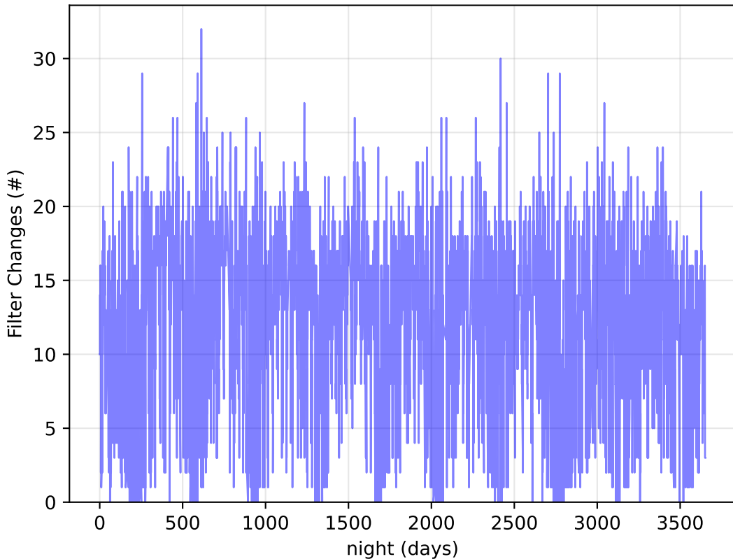
weather_cloudso18v3.4_10yrs Per Night: Filter Changes
